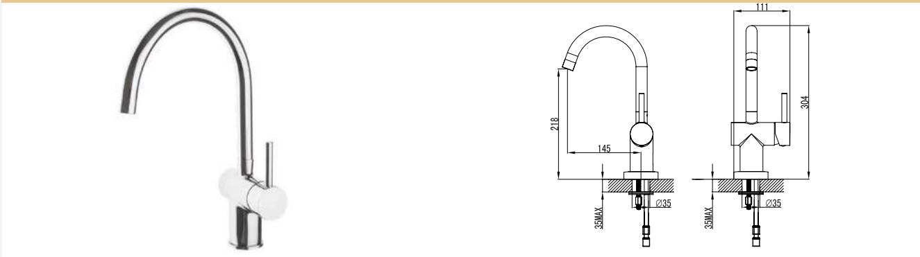
92100 Adorn Elegance Sink Mixer
