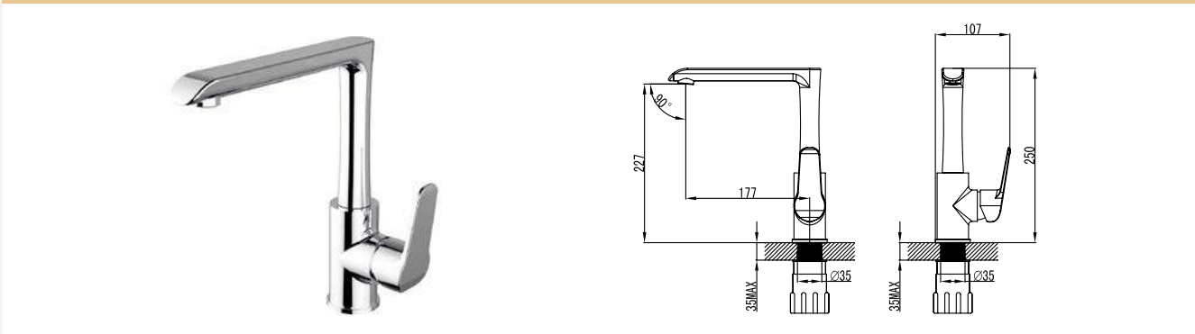
92104 Start Elegance Sink Mixer
