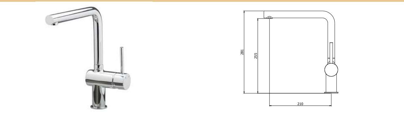
4G4175 Horizontal Spout Sink Mixer
